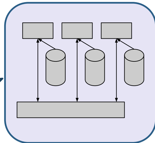
Microservices + Events
